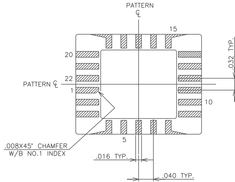
BONDING PATTERN
