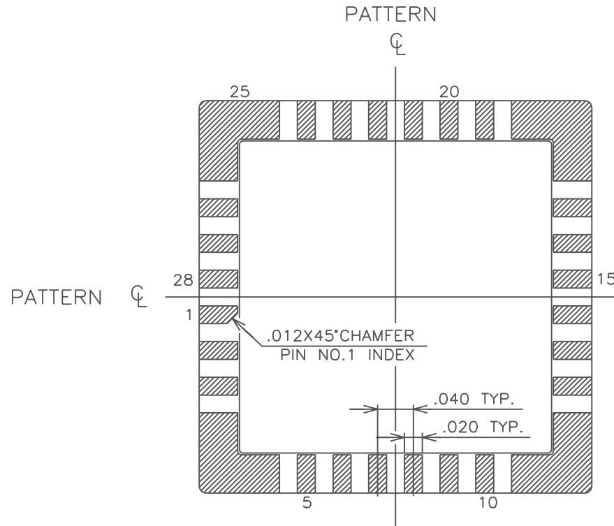
BONDING PATTERN
