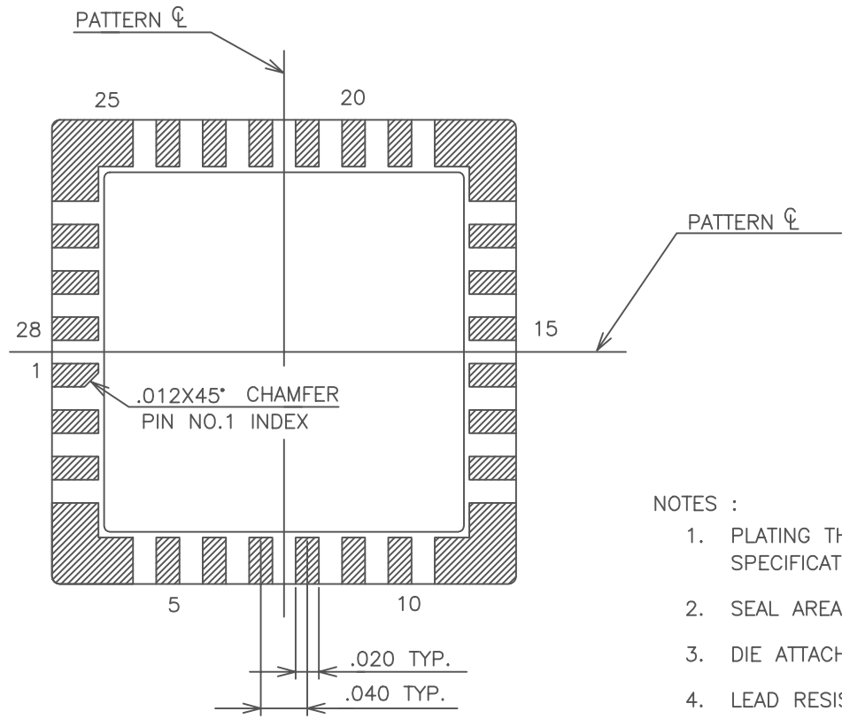
BONDING PATTERN
