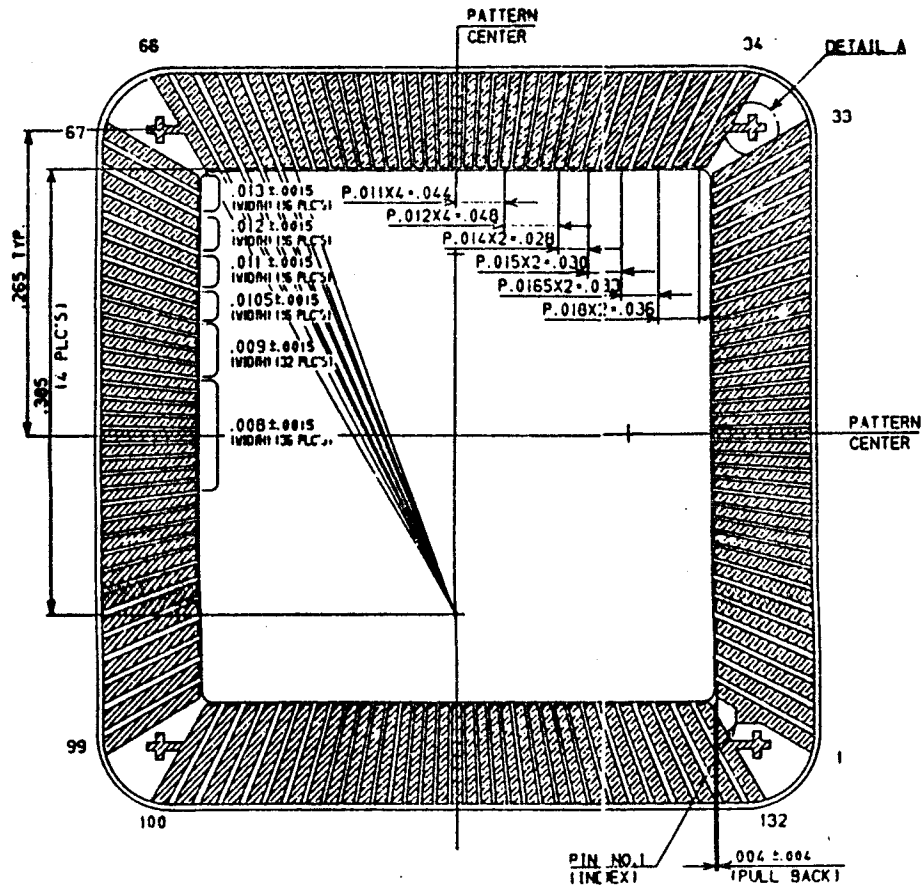
DETAIL OF WIRE BONDING AREA
