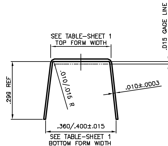
FORMING DIMENSIONS 5X SCALE
