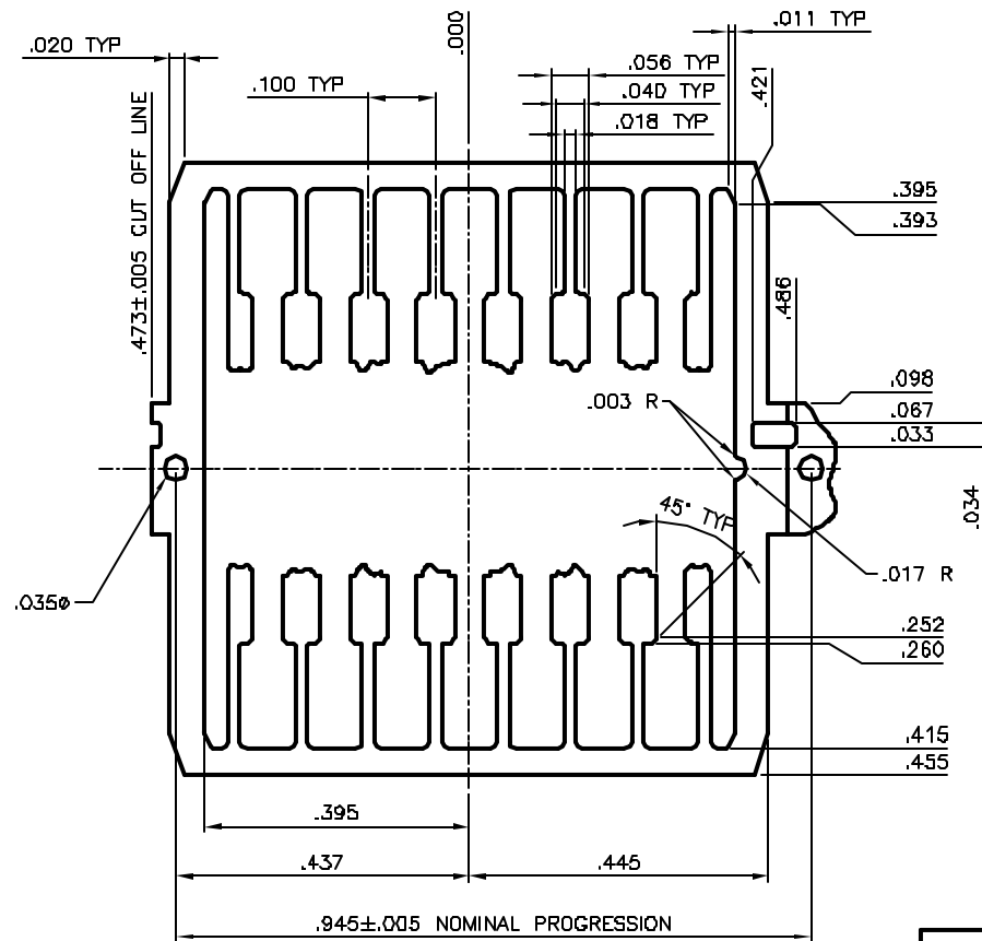
EXTERNAL FRAME CONFIGURATION "A" 5X SCALE
