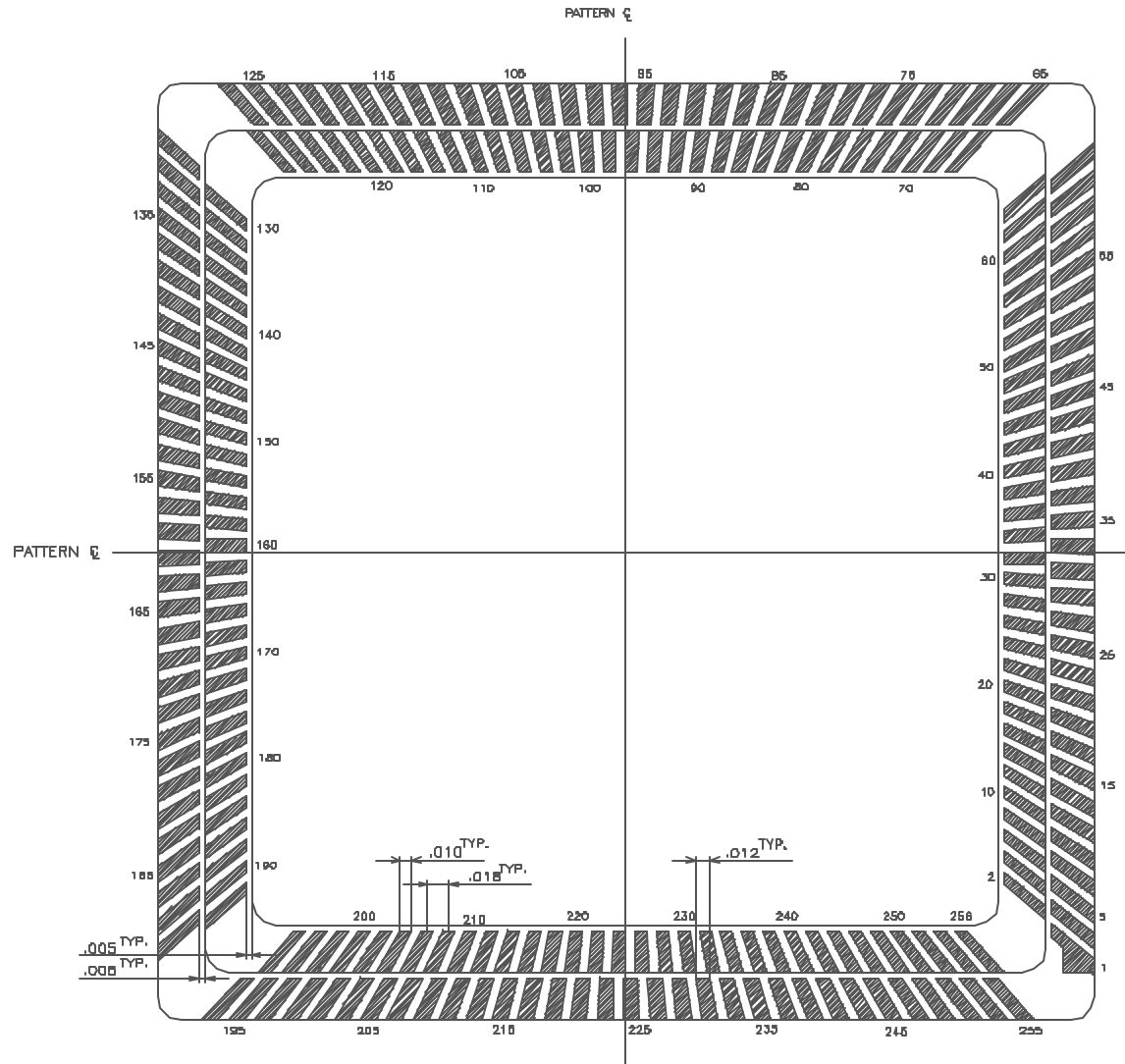
BONDING PATTERN
