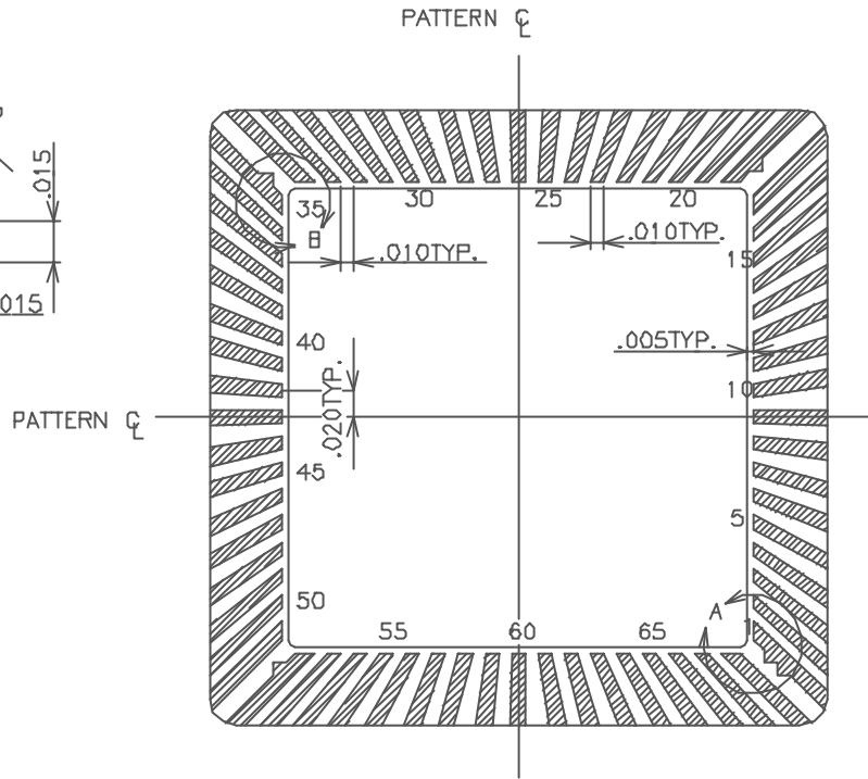
BONDING PATTERN
