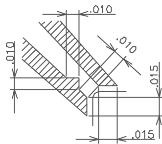
DETAIL-B (3PLCS)
