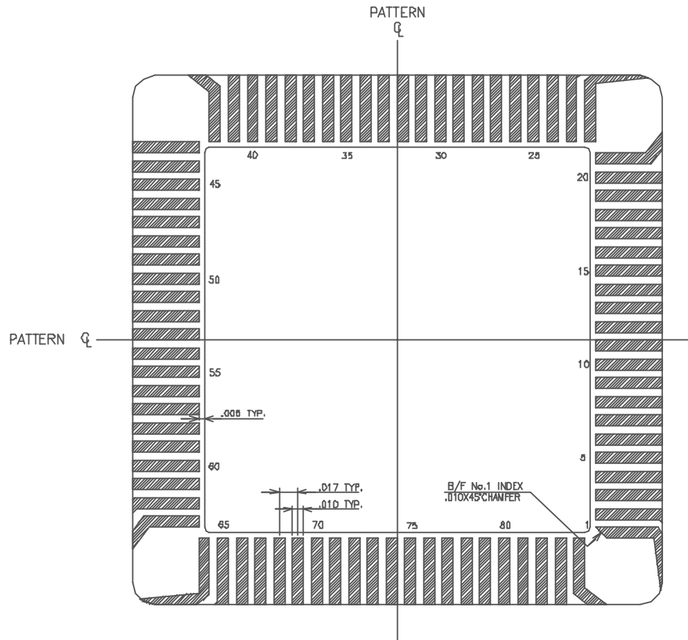
BONDING PATTERN
