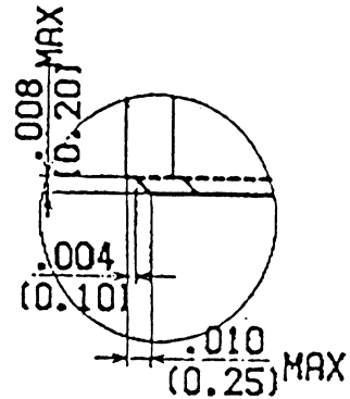
VIEW "P"
