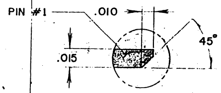
VIEW IN CIRCLE -Z- (ENLARGED)
