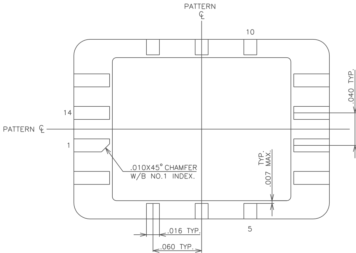
BONDING PATTERN
