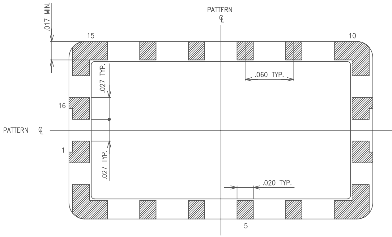
BONDING PATTERN
